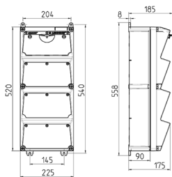
Drawing 1 MB 523
